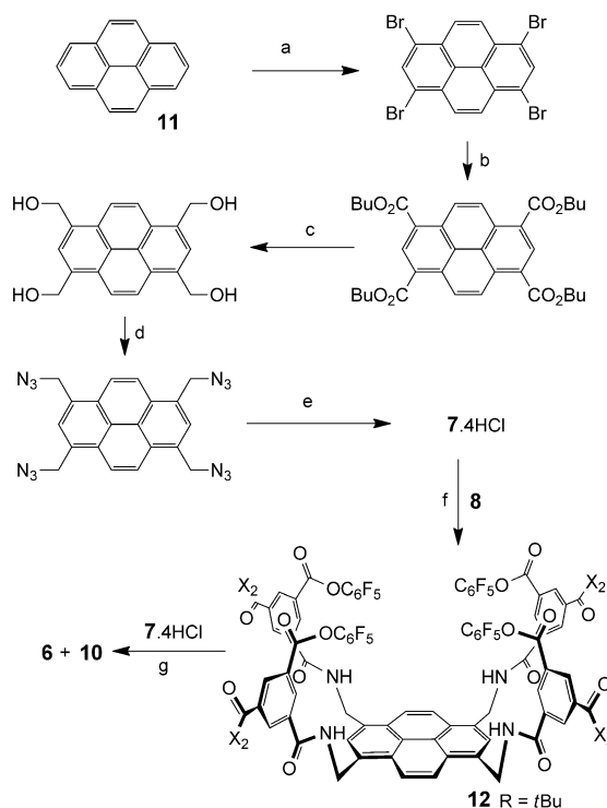
Scheme 1. Synthesis of the protected receptors 6 and 10 . Reaction conditions: a) Br 2 , PhNO 2 , 96%; b) BuOH, CO (30 bar), DIPEA, Pd(OAc) 2 , BINAP, xylenes, 89%; c) LiBH 4 , THF, MeOH, ca. 100%; d) (PhO) 2 PON 3 , DMF, DBU, 52%; e) Ph 3 P, THF, H 2 O; then HCl (aq.), 93%; f) DIPEA, H 2 O, THF, 47%; g) DIPEA, H 2 O, THF, 57%.
